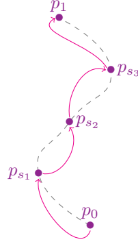
Figure 6: The dashed curve is the path of steady states (for instance in W^{1,2}(\Omega) \cap \mathcal{C}^0(\overline{\Omega}) ), and the points are the close enough steady states. We represent the exact control in finite time T_1 > 0 with the pink arrows.
